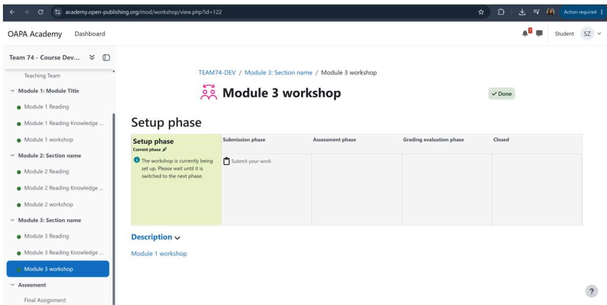
Fig. 8. Module 3 Workshop marked Done. Its description also incorrectly reads "Module 1 workshop," the same copy-paste mistake seen on Module 2, so this looks like one shared issue rather than two separate ones.
